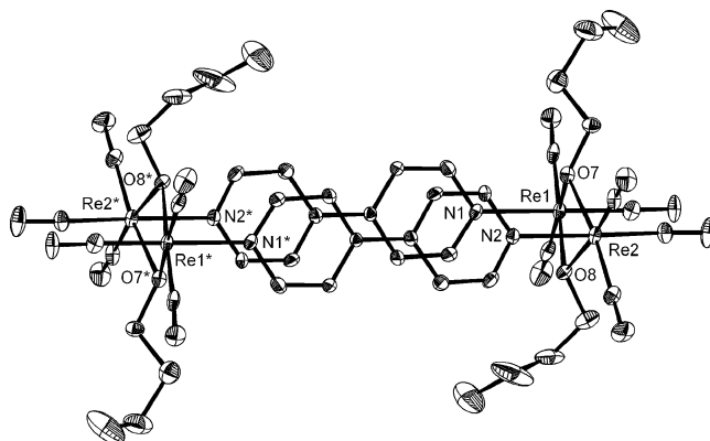
Figure 2. ORTEP plot of 1 . Hydrogen atoms and disordered butoxy carbon atoms have been omitted for clarity. The thermal ellipsoids represent 30% occupancy. Selected bond lengths [ \text{ \AA} ]: Re1–C1, 1.878(10); Re1–C2, 1.895(10); Re1–C3, 1.912(10); Re1–O7, 2.141(5); Re1–O8, 2.139(5); Re1–N1, 2.218(6); Re2–C4, 1.896(9); Re2–C5, 1.890(10); Re2–C6, 1.916(9); Re2–O7, 2.141(5); Re2–O8, 2.148(5); Re2–N2, 2.227(6).
